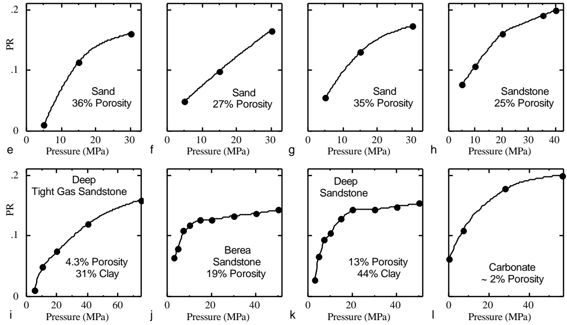
Figure 3. PR versus differential pressure in room-dry samples. Data used are from Nur (1969), Yin (1993), Han (1986), Blangy (1992), and authors' database.
